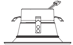
S11638: 4" (101mm)
