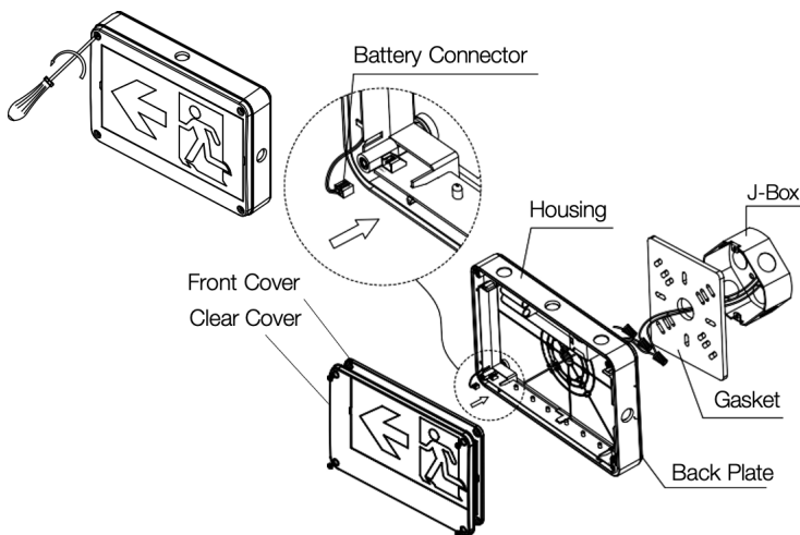
Figure 1 - Wall Mount
