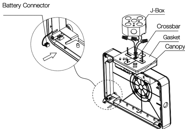
Figure 3 - Ceiling Mount
