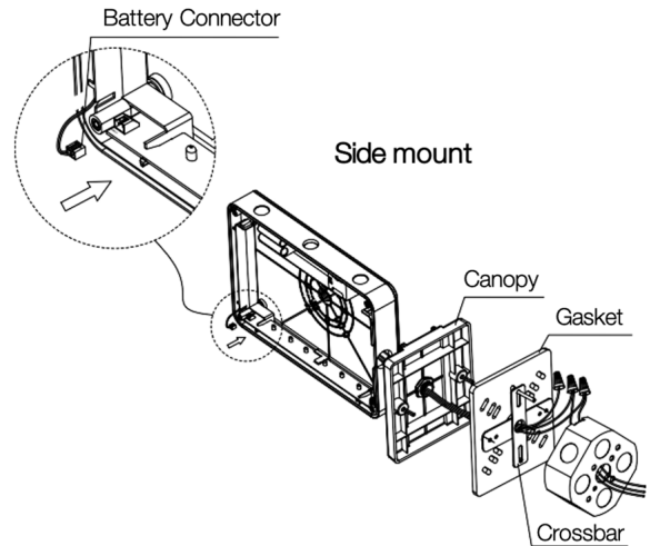
Figure 2 - Side Mount
