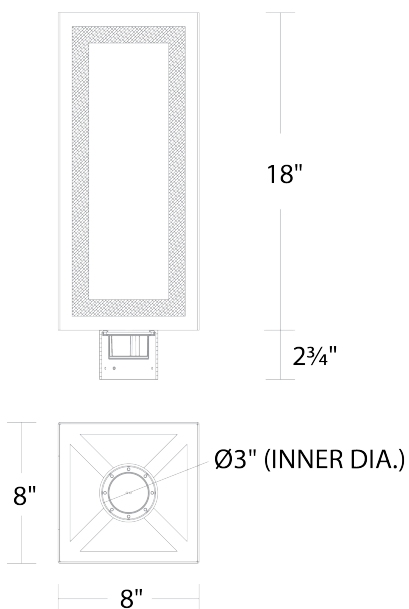
PM-W24521
