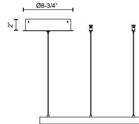
Side Canopy Option
