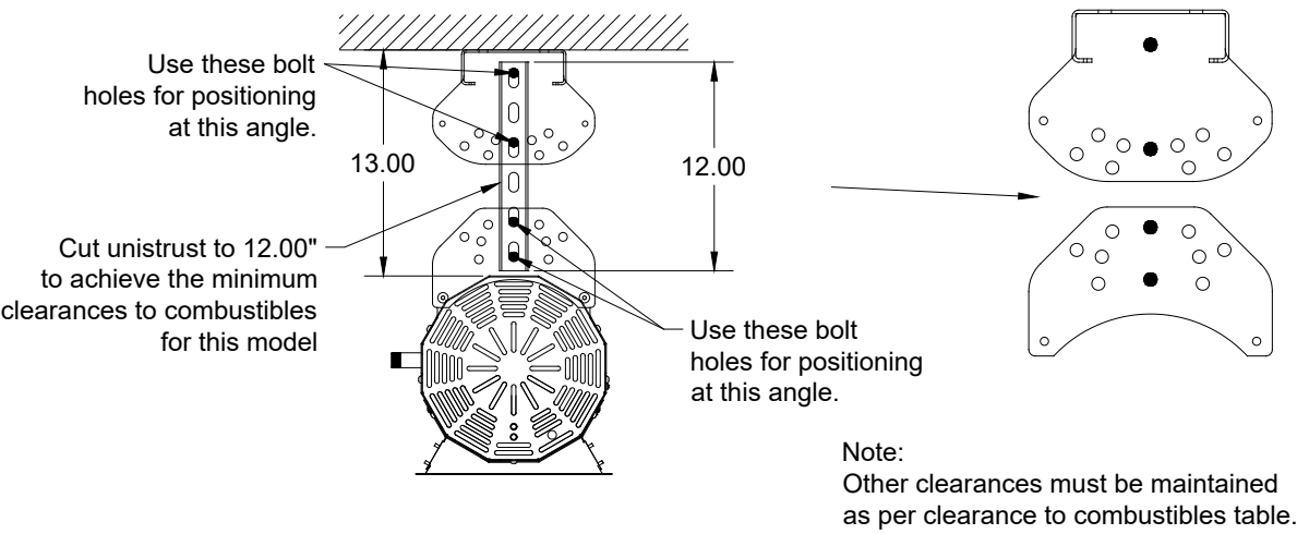
Minimum Ceiling Mount Distance using Optional Shield
