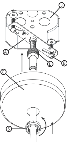
Drawing 2– Mounting Detail
