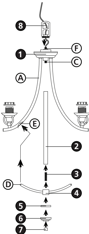
Drawing 2 - Glass Installation
