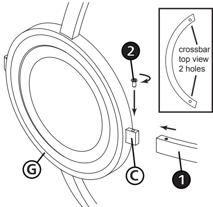
DRAWING 3 - ASSEMBLY
