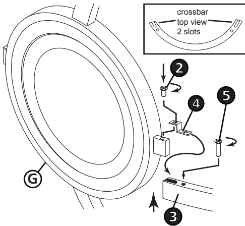
DRAWING 3 - ASSEMBLY
