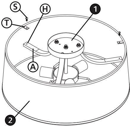
DRAWING 2 - STRAP DETAIL
