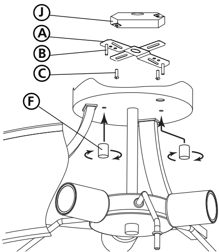
DRAWING 3 - INSTALLATION
