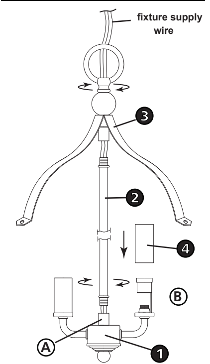
Drawing 1 - Cage Assembly
