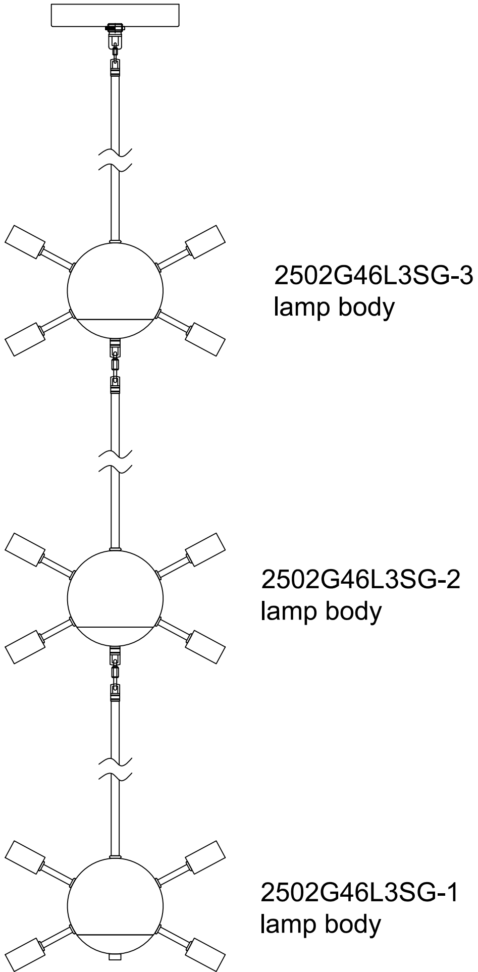
Schematic diagram of three-layer lamp body assembly
