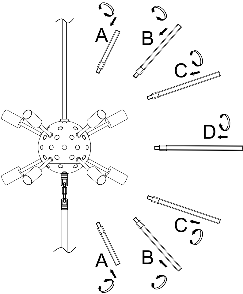
Schematic diagram of layer installation
