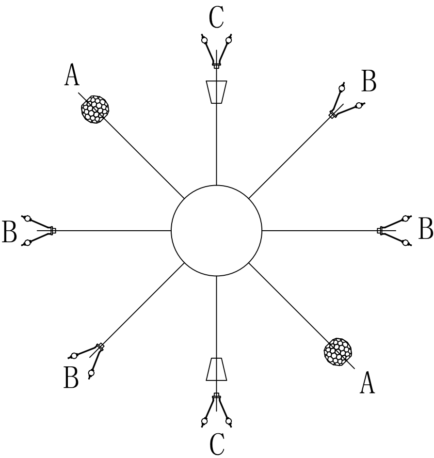
layer 6 Installation diagram
