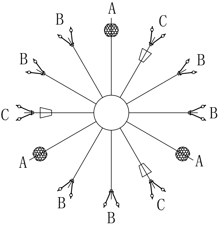
layer 4 Installation diagram
