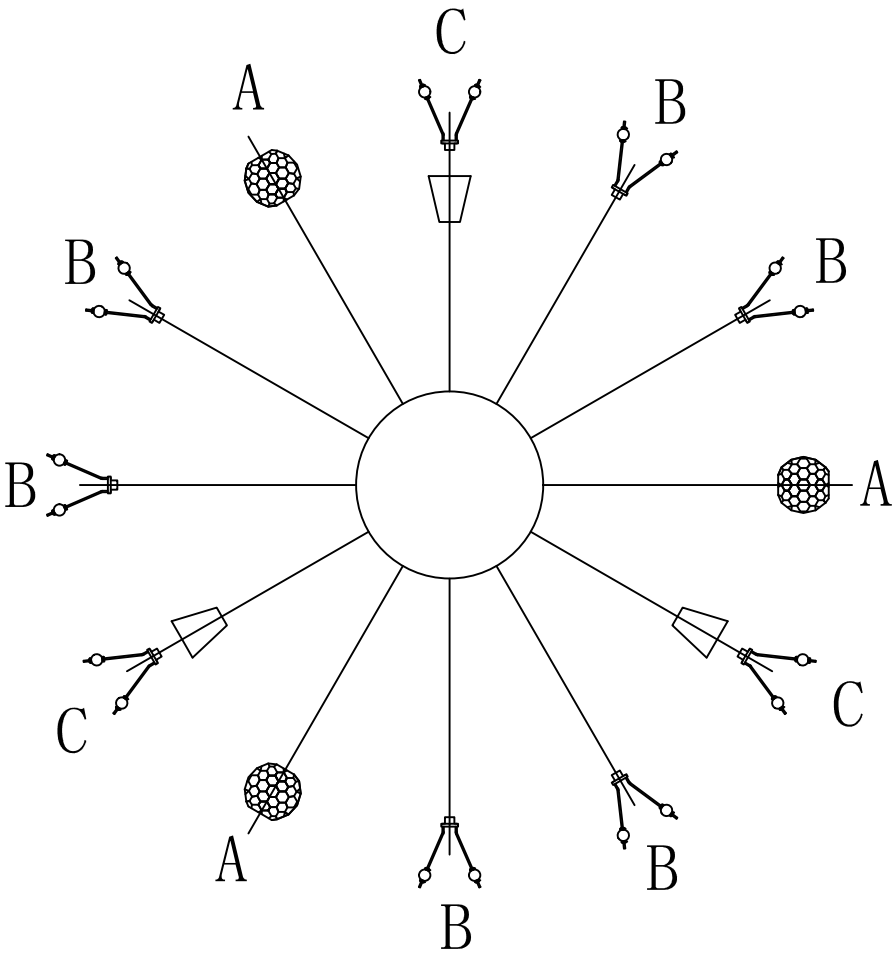
layer 5 Installation diagram
