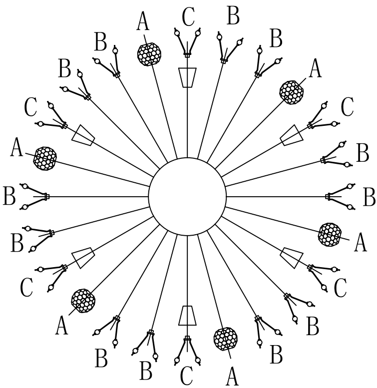
layer 1 Installation diagram
