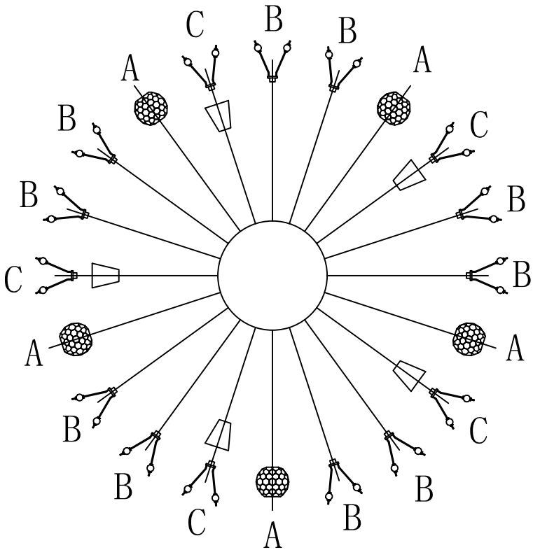
layer 2 Installation diagram
