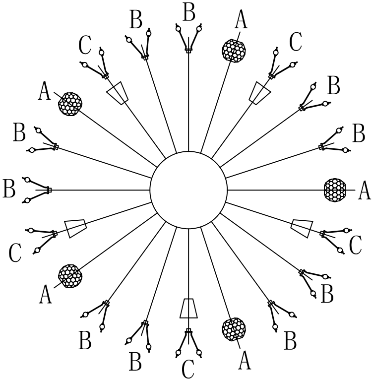
layer 3 Installation diagram
