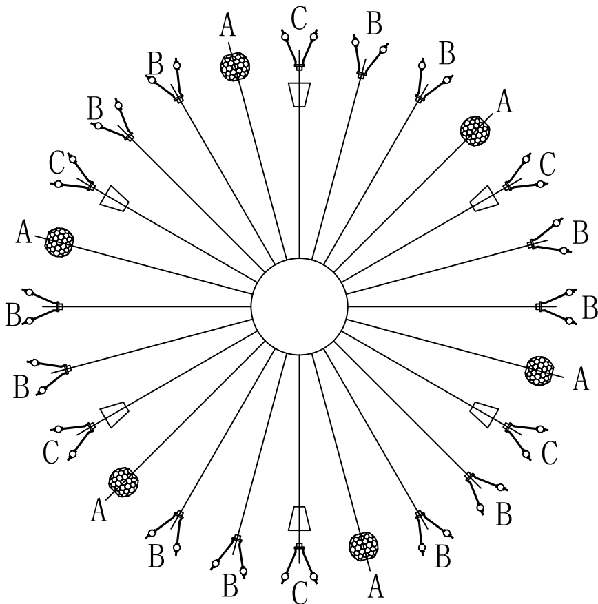
layer 2 Installation diagram
