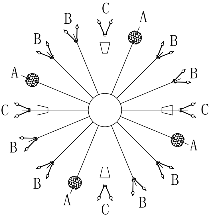
layer 3 Installation diagram
