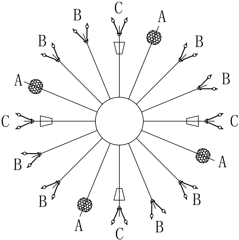
layer 4 Installation diagram
