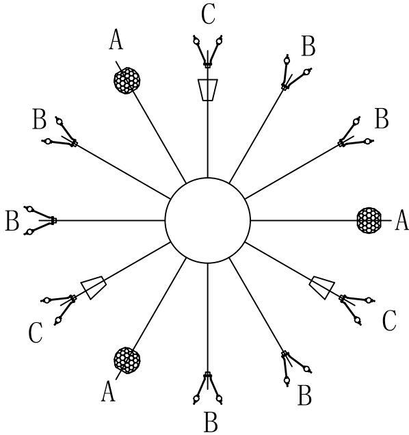
layer 5 Installation diagram
