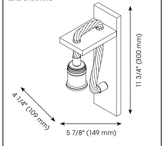
LINE DRAWING
