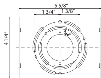
Mounting Plate Dimensions
