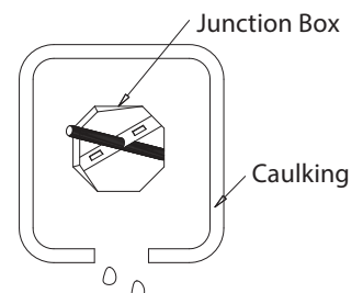
Fig. 4 Sealing
