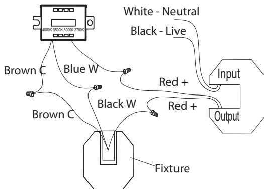
Fig. 3 Driver Wires
