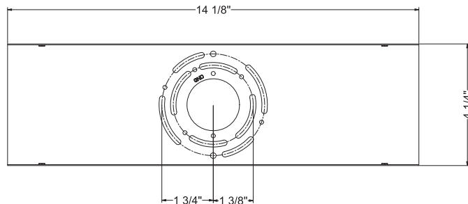
Back Plate Dimensions
