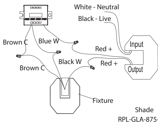
Fig.3 Driver Wires
