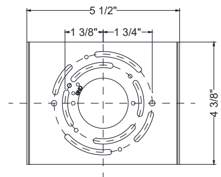
Mounting Plate Dimensions
