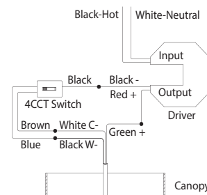
Fig. 4 Driver Wires
