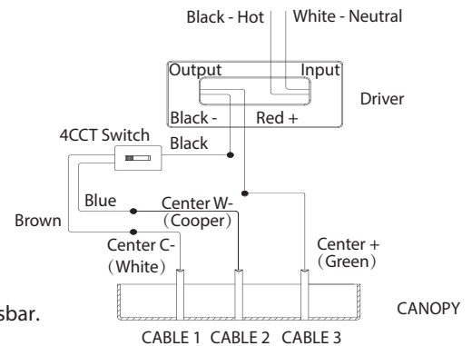
Fig.5 Driver Wires
