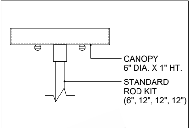
CANOPY DETAIL
