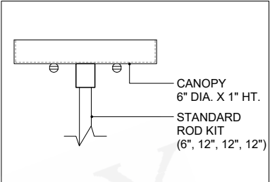
CANOPY DETAIL
