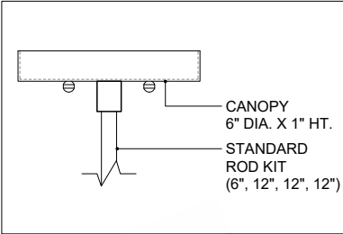
CANOPY DETAIL
