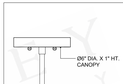
CANOPY DETAIL
