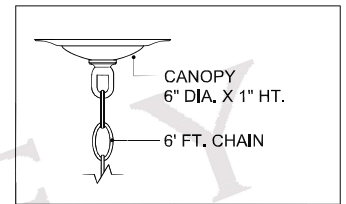
CANOPY DETAIL
