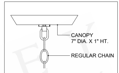
CANOPY DETAIL
