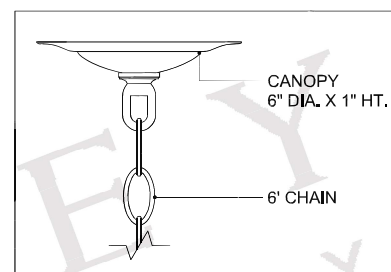
CANOPY DETAIL
