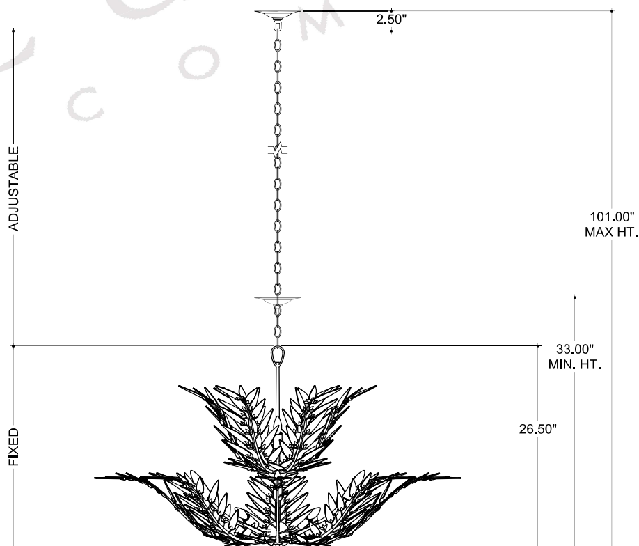
FRONT VIEW
