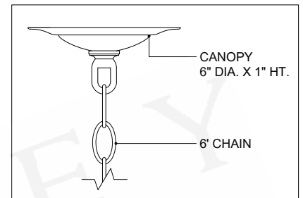
CANOPY DETAIL
