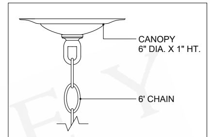
CANOPY DETAIL
