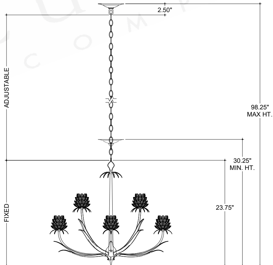
FRONT VIEW
