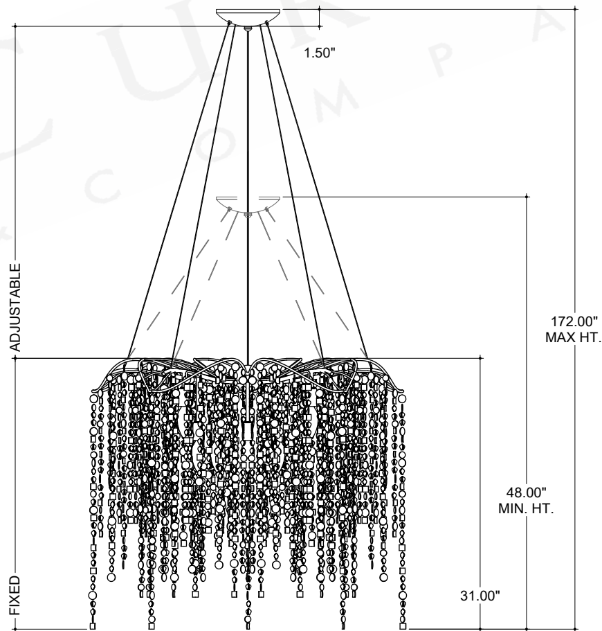
FRONT VIEW
