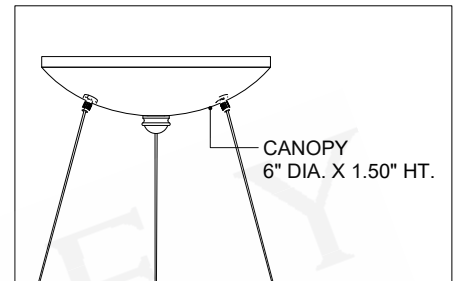
CANOPY DETAIL
