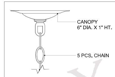
CANOPY DETAIL
