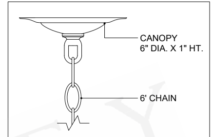
CANOPY DETAIL
