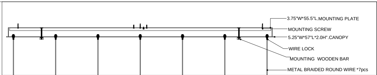
CANOPY DETAIL
