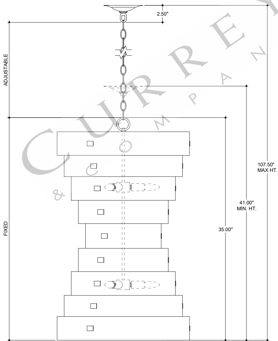
FRONT VIEW
