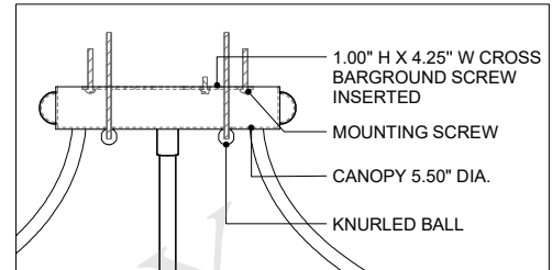
SEMI-FLUSH CANOPY DETAIL
