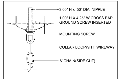
CHANDELIER CANOPY DETAIL
