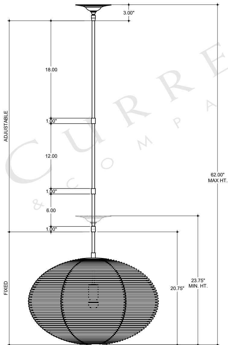
FRONT VIEW
