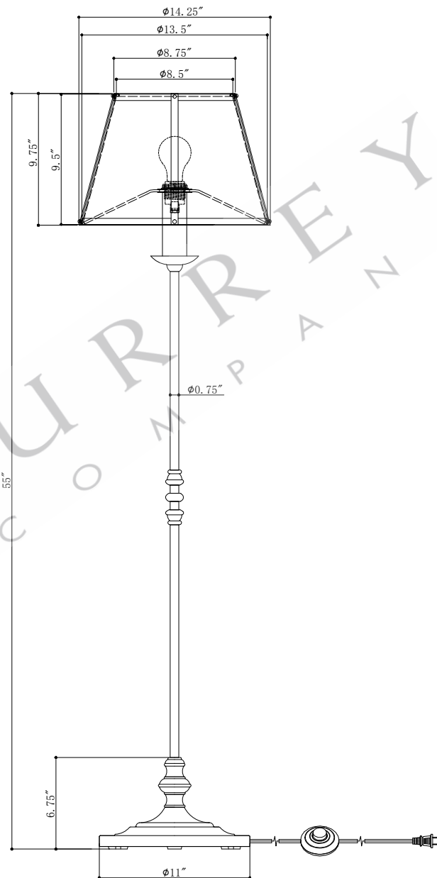
FRONT VIEW
