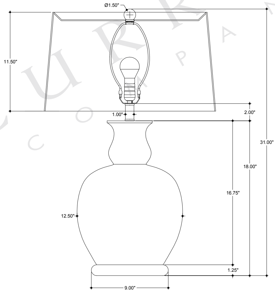
FRONT VIEW
