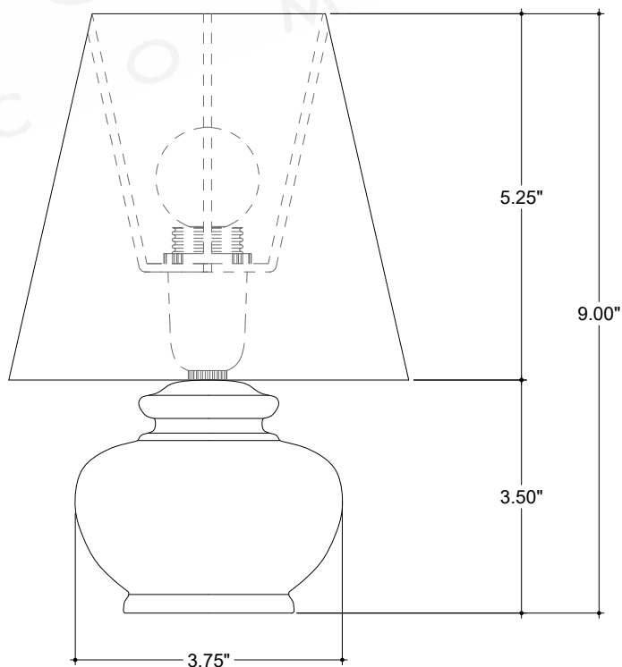
FRONT VIEW
