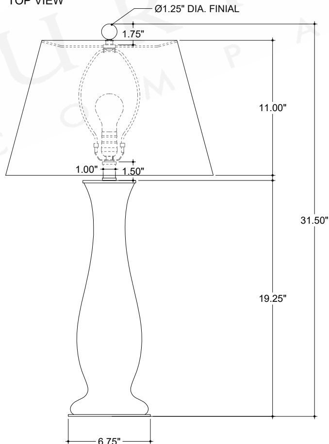
FRONT VIEW
