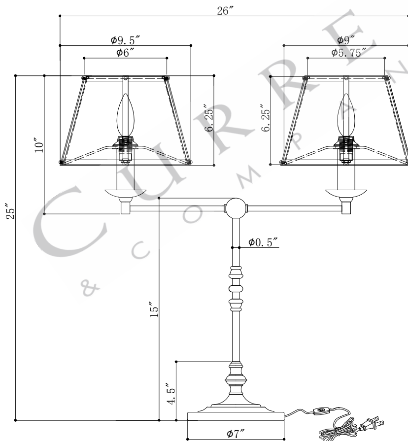
FRONT VIEW
