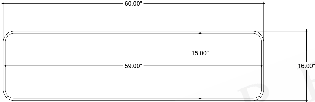
TOP VIEW
