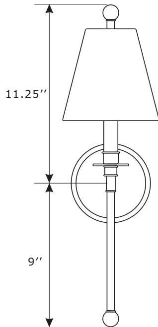
FRONT VIEW WITH LONG ROD
