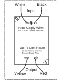
Wiring diagram
