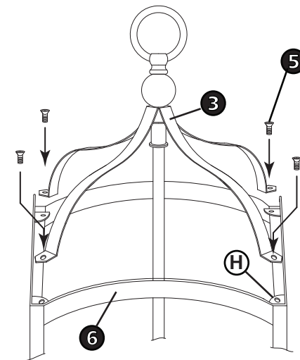
Drawing 2 - Cage Assembly
