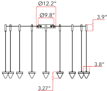
Front Elevation
