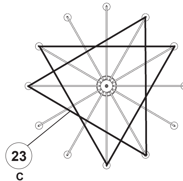
DIAGRAM 2 (BOTTOM VIEW)
