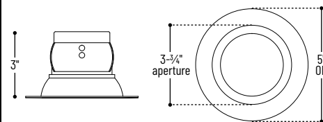
NOXTW-431WW / NOX-4BAFB Black Baffle Insert
