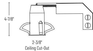
NHR10IC-16LE4 1" Iolite IC Air-Tight Remodel Housing
