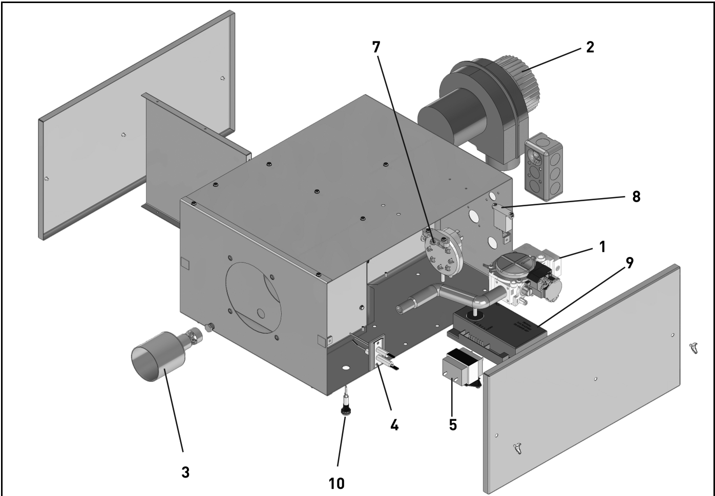
FIGURE 32: Burner Exploded View
