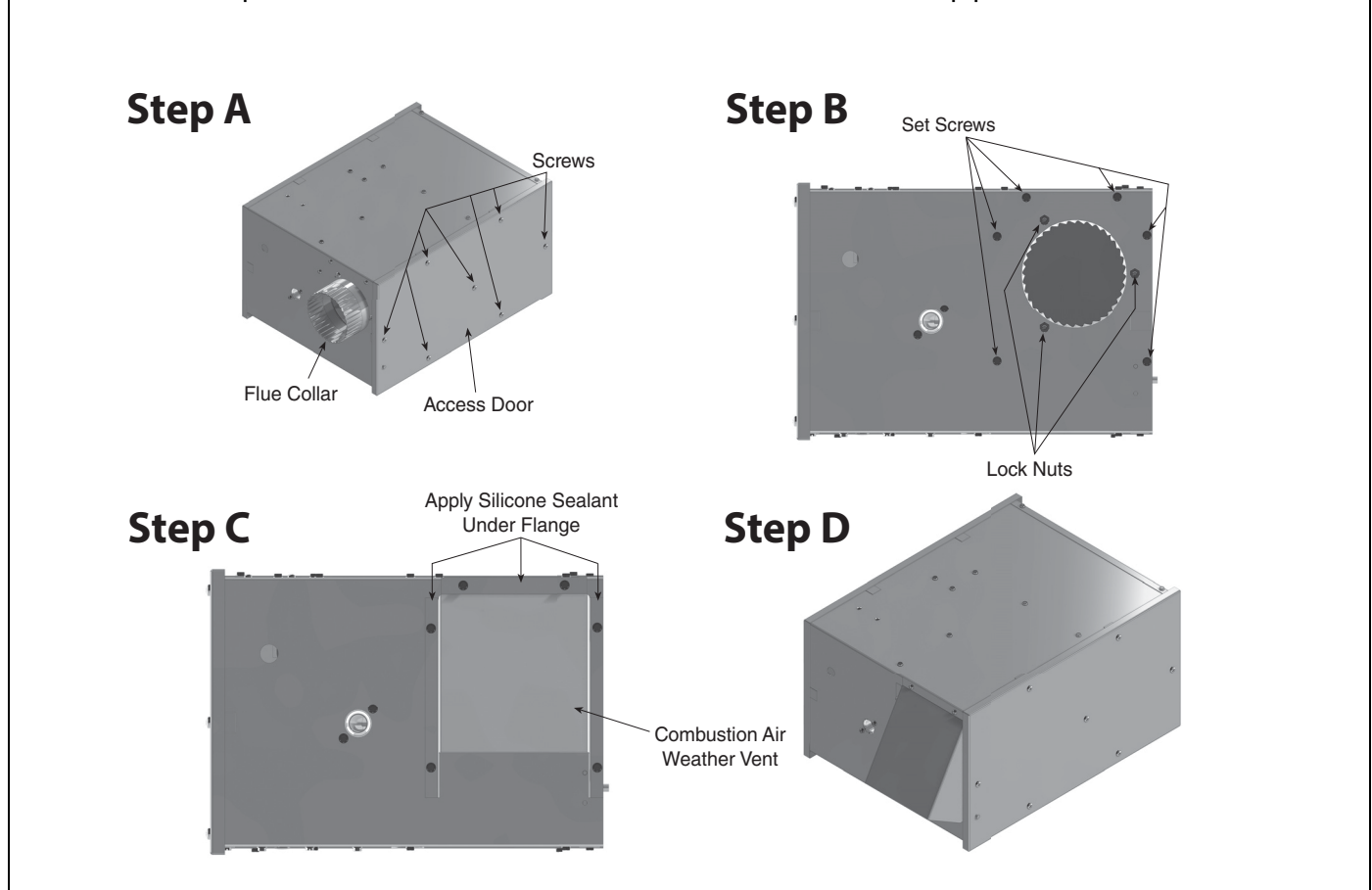
FIGURE 30: Combustion Air Weather Vent (P/N 03700009)
