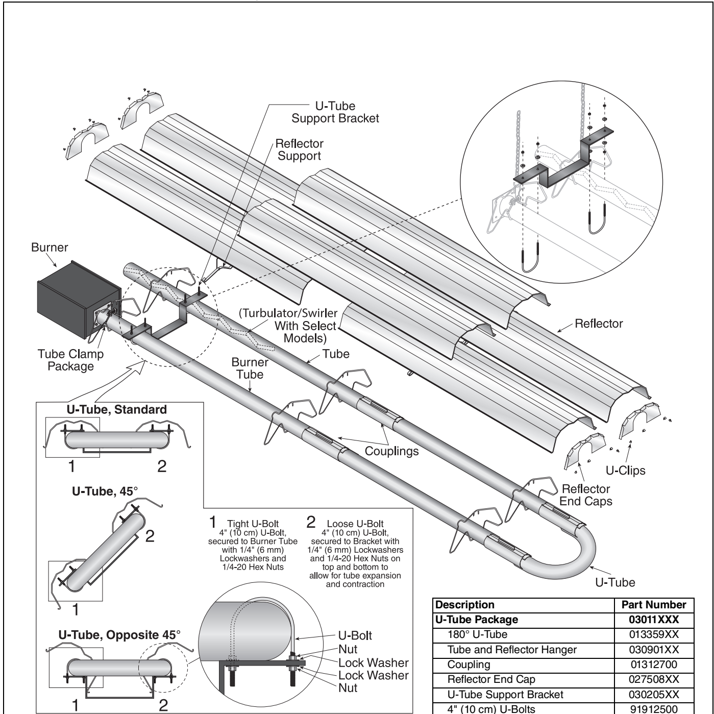
FIGURE 25: U-Tube Heater Assembly Overview
