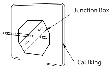
Fig.3 Sealing
